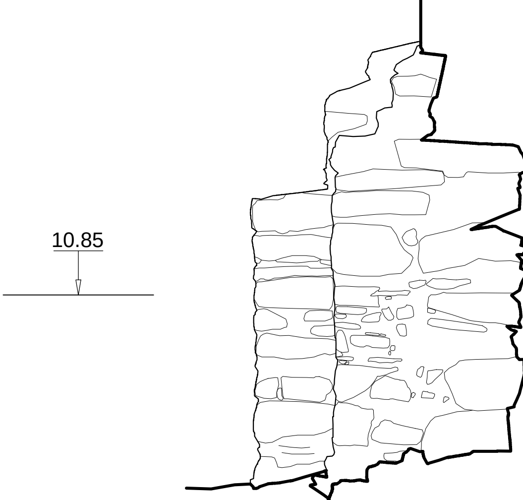
FACADE E
